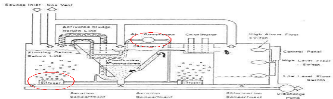
(Fig. 1) "SASAKURA SUPER TRIDENT" SEWAGE TREATMENT PLANT
