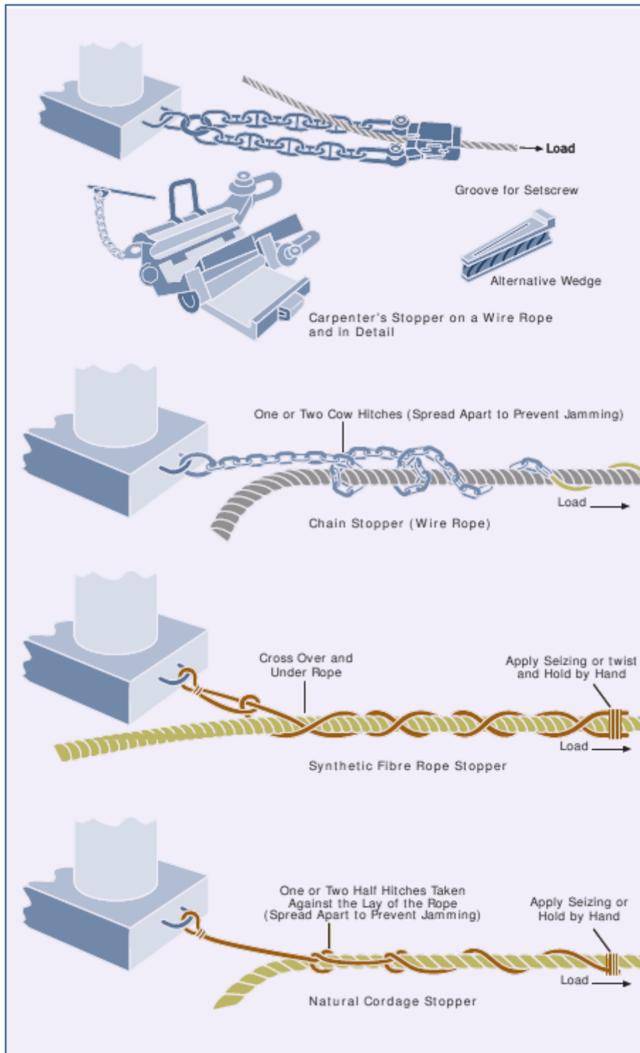
Figure 8.6: Stoppers
